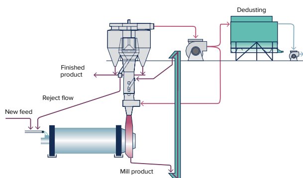
SEPAX system for raw grinding installation suitably integrated into the mill vent line.
