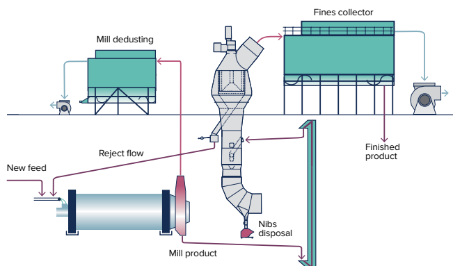
SEPAX system with bag filter for collection of fines: This system ensures maximum product cooling.
