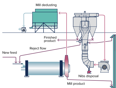
SEPAX system with cyclones for collection of fines: Lowest initial and operating costs. Recuperation of heat enhances drying of wet slag, puzzolana or other additives.
